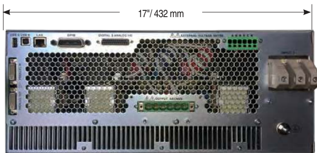
The AFX Rear Panel provides connections for AC Input, AC or DC Output, External Sense, Aux I/O and remote control interfaces. Shown here with optional GPIB Interface
