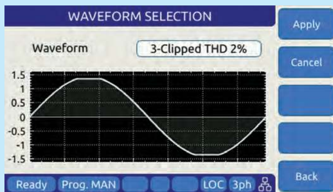
AC Waveform Selection - Vthd = 2%
