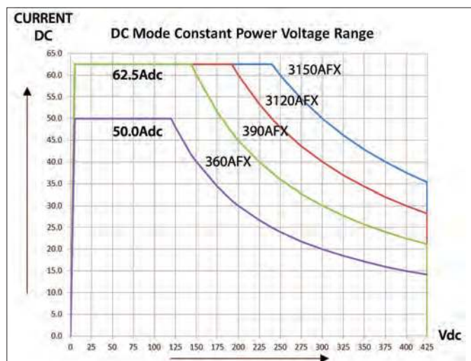
DC current vs. Voltage for 360AFX ~ 3150AFX models in single phase mode
