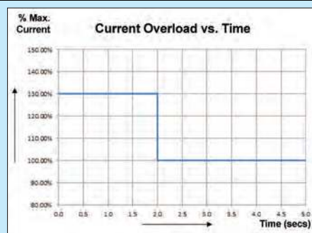
Current Overload Mode Profile
