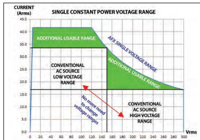
Extended Operating Range for model 3150AFX along Constant 5 kVA per Phase Power Curve. Other models have same profile but other current levels.
